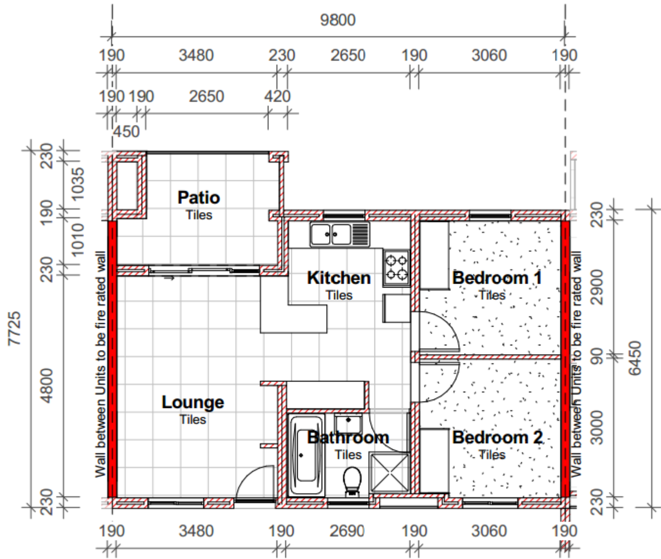
Floor Plan: Unit Type B
