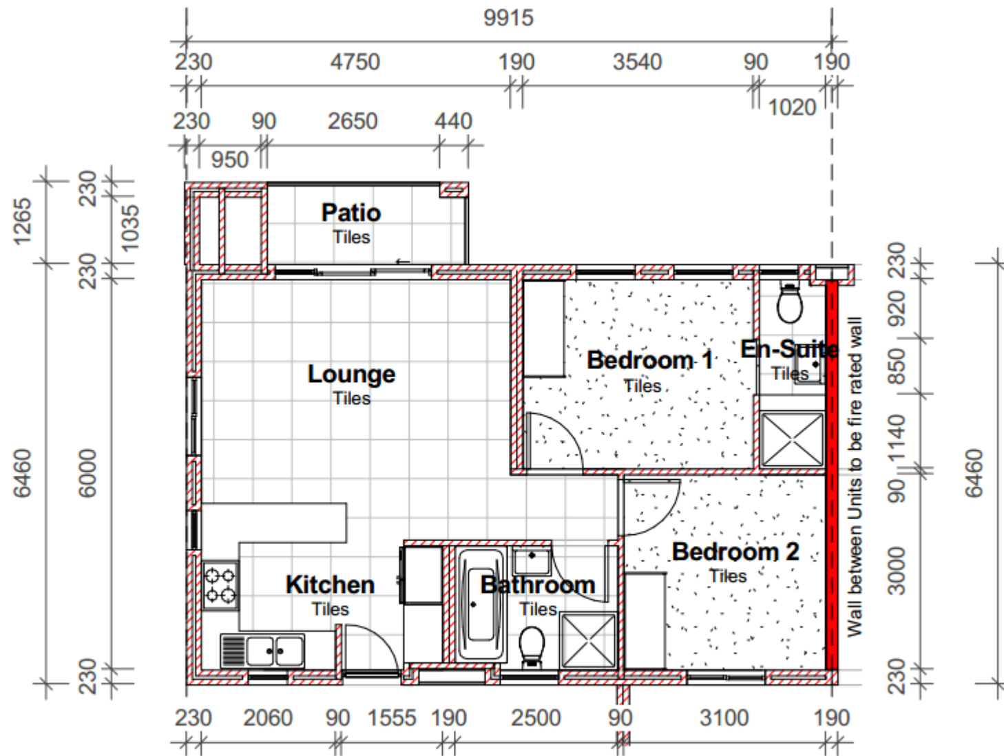
Floor Plan: Unit Type A1
